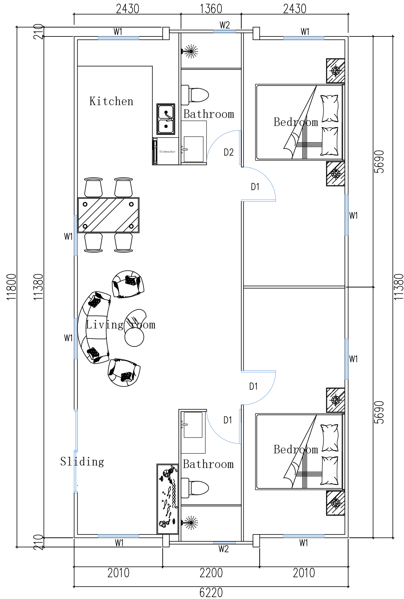
40ft 2bedrooms 1Living room 2bathrooms
