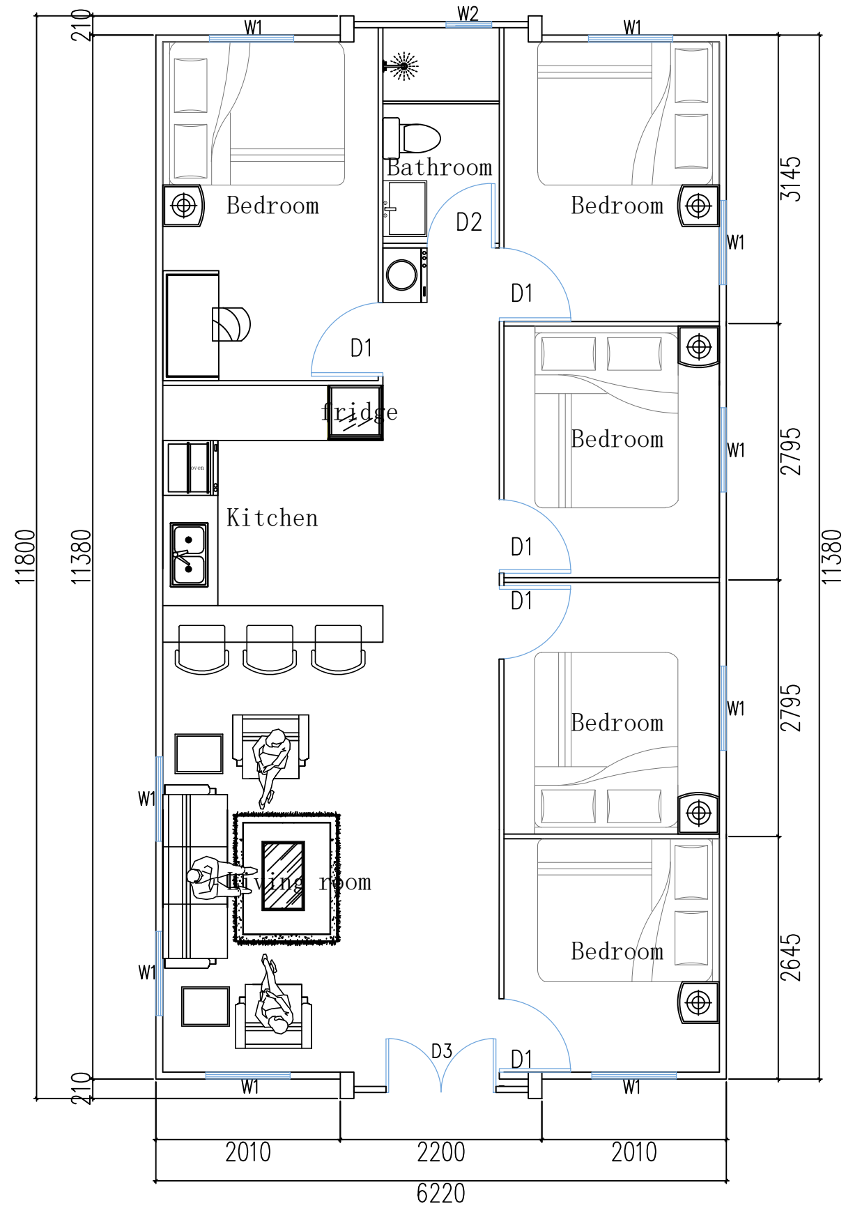
40ft 5bedrooms 1Living room 1bathroom
